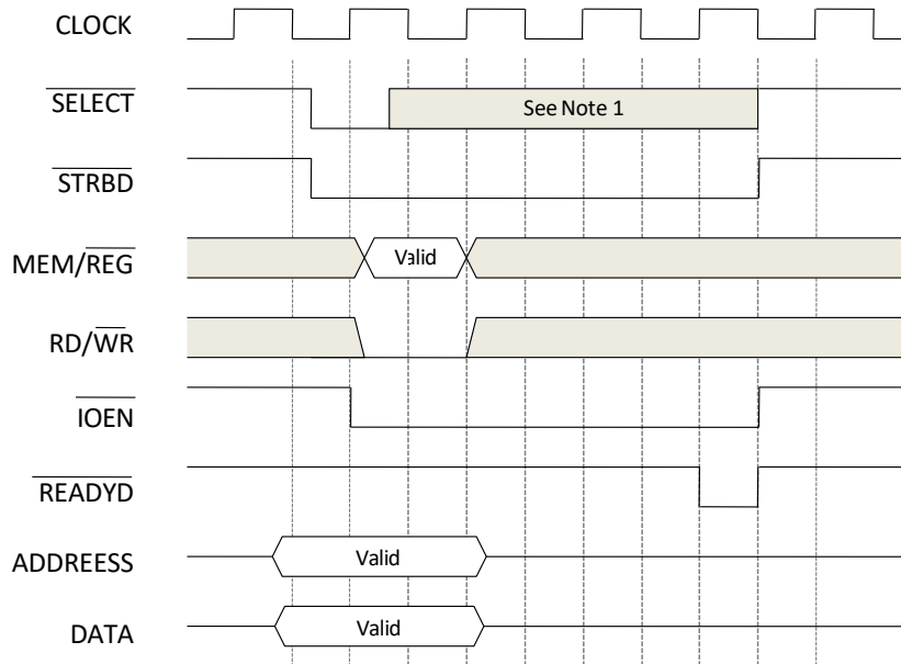
Figure 3: Write Cycle
