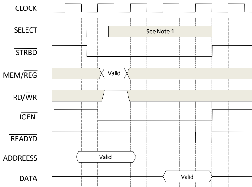
Figure 4: Read Cycle
