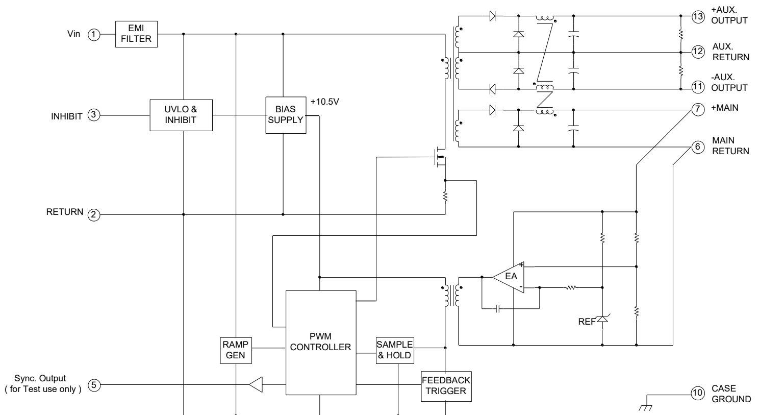
Figure 1. Block Diagram
