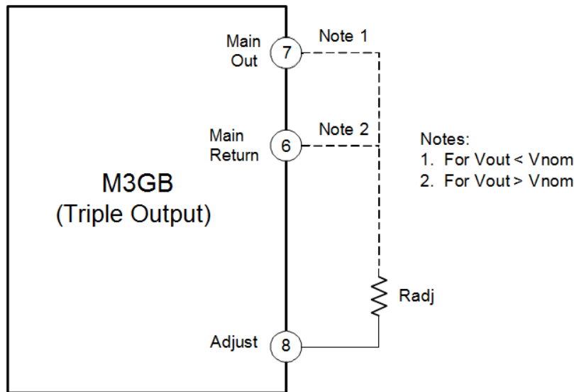
Fig 4. Configuration for Adjusting Triple Output Voltage
