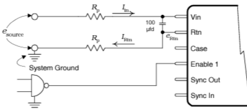
Figure 6. Problems of Parasitic Resistance in Input Leads
