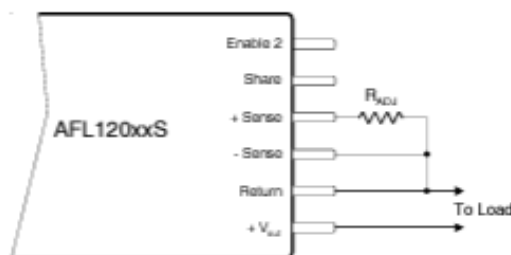
Figure 5. Connection for V_{OUT} Adjustment
