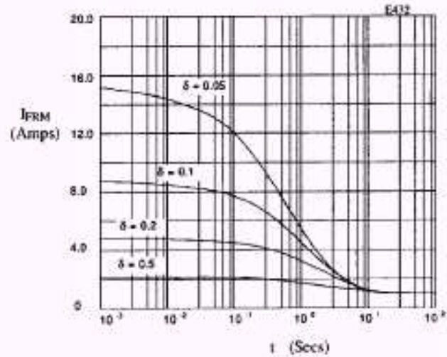
Fig 8. Typical repetitive forward current as a function of pulse width at 100°C; R_{\theta JL} = 80^\circ\text{C/W} ; V_{RWM} during 1 - \delta .
